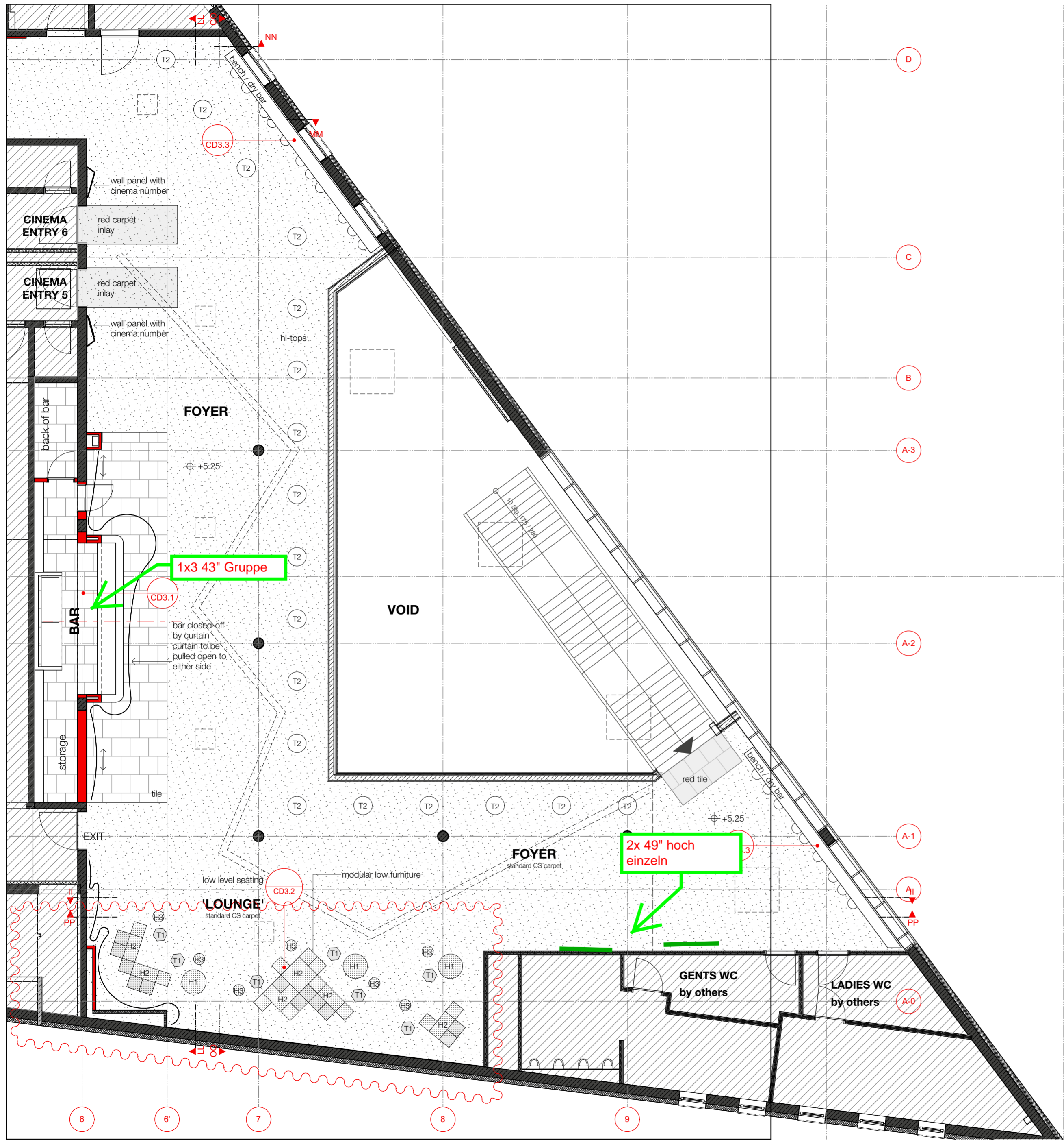
1 FIRST FLOOR FURNITURE PLAN 1:100
