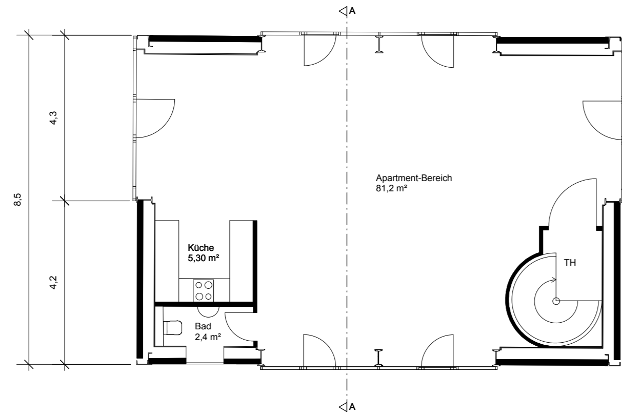
Hotel-Apartment 2.OG
