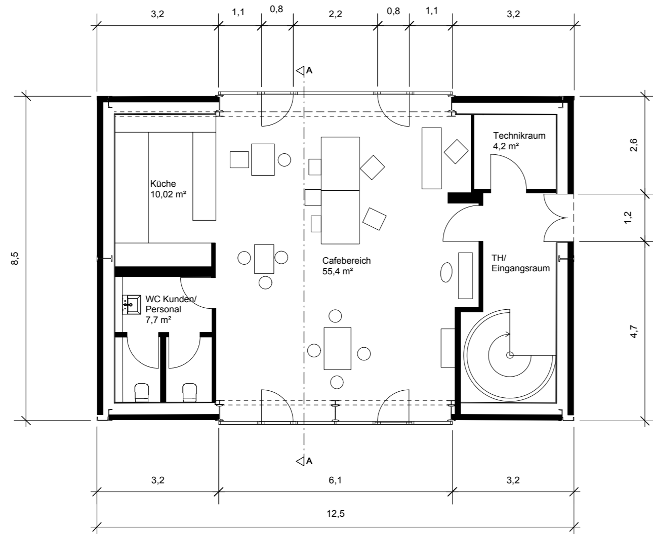
Cafe EG
